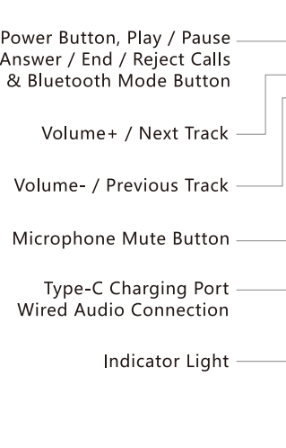
ALL-in-One Wireless Headset
